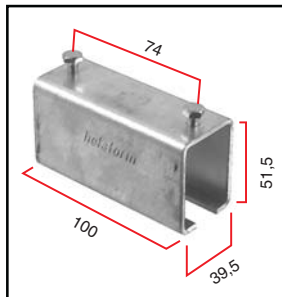
Joint LK-102 100 mm
