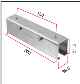
Joint LK-102 200 mm
