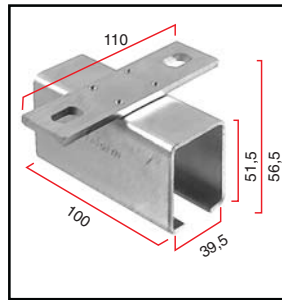
Soffit bracket KKK-102
