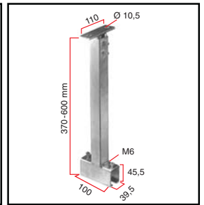
Soffit bracket KKS-102
