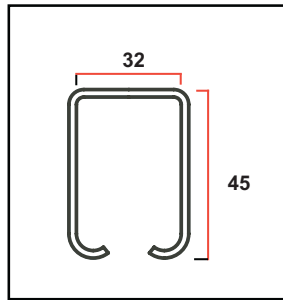
Track K-102, profile
